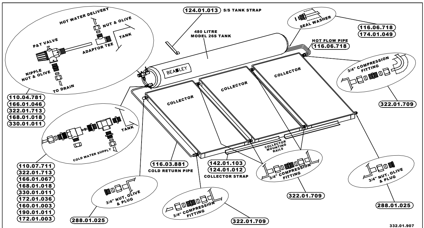
Figure 10.480 Litre Three Collector System
