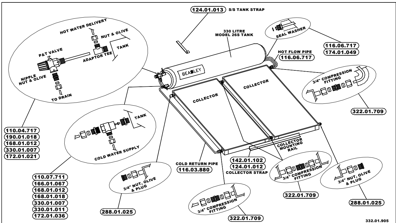
Figure 8. 330 Litre Two Collector System
