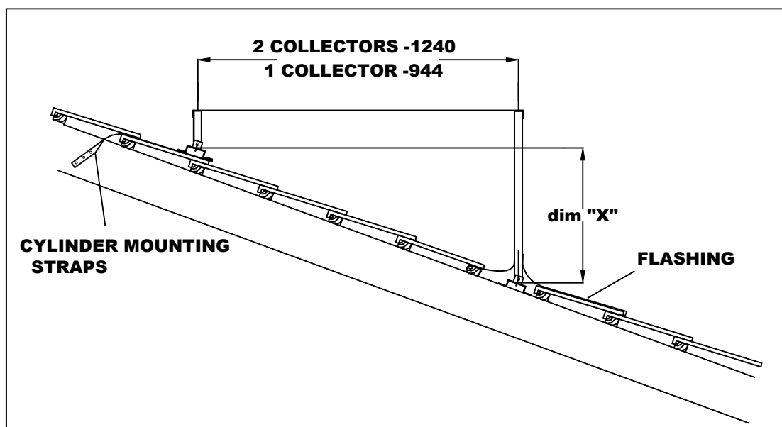
Figure 18. Frame Dimensions
