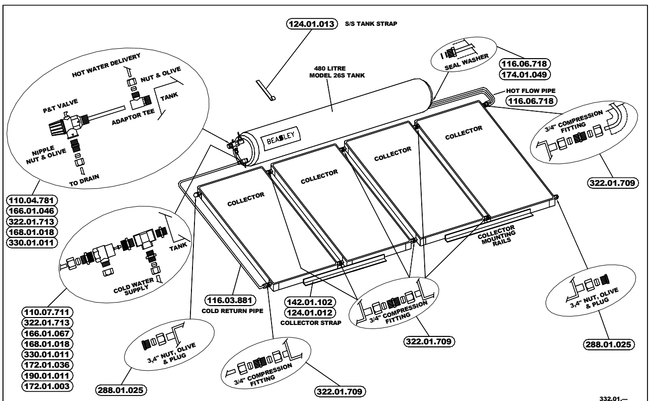
Figure 11.480 Litre Four Collector System
