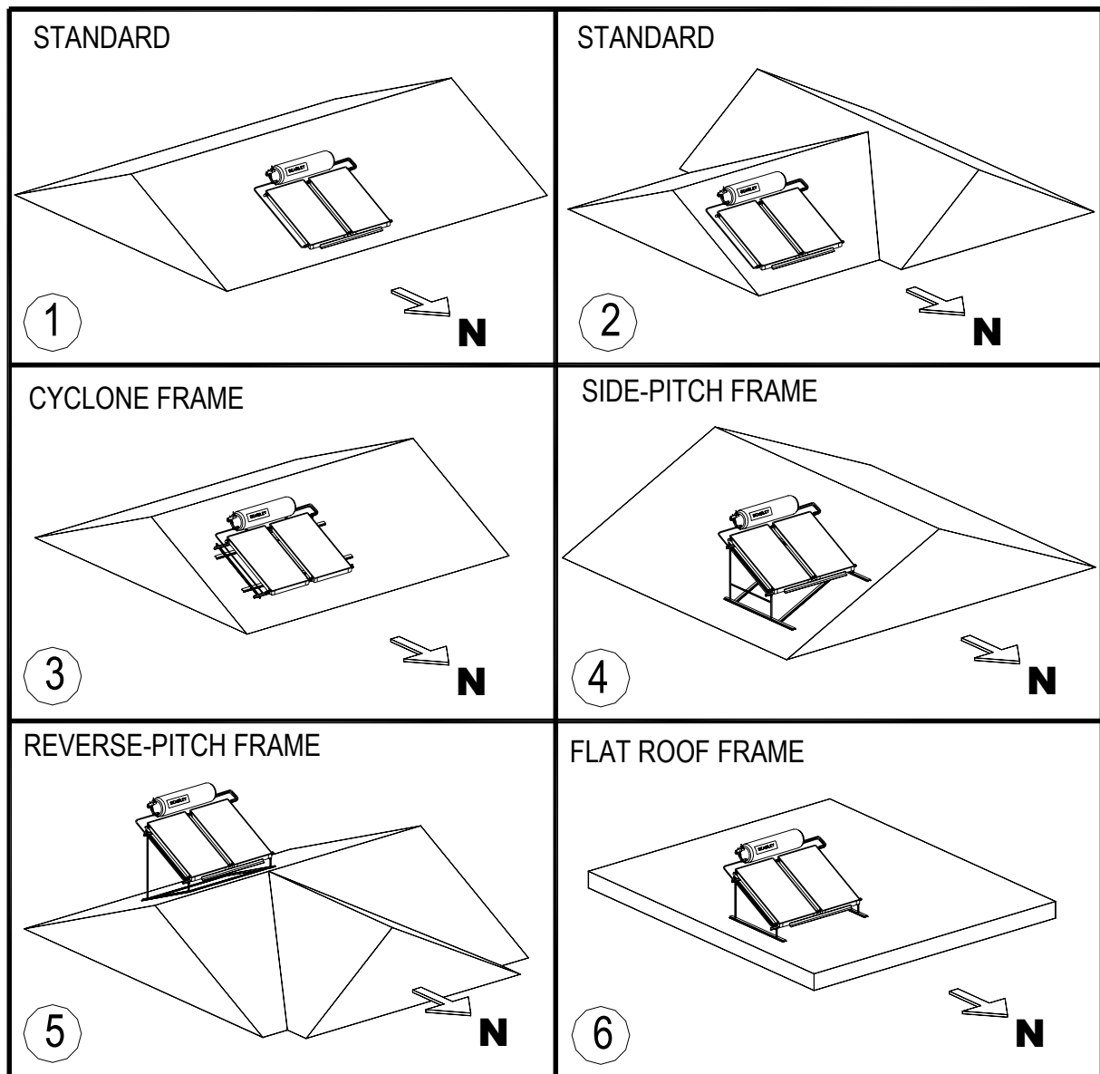
Figure 5. System Mounting Options
