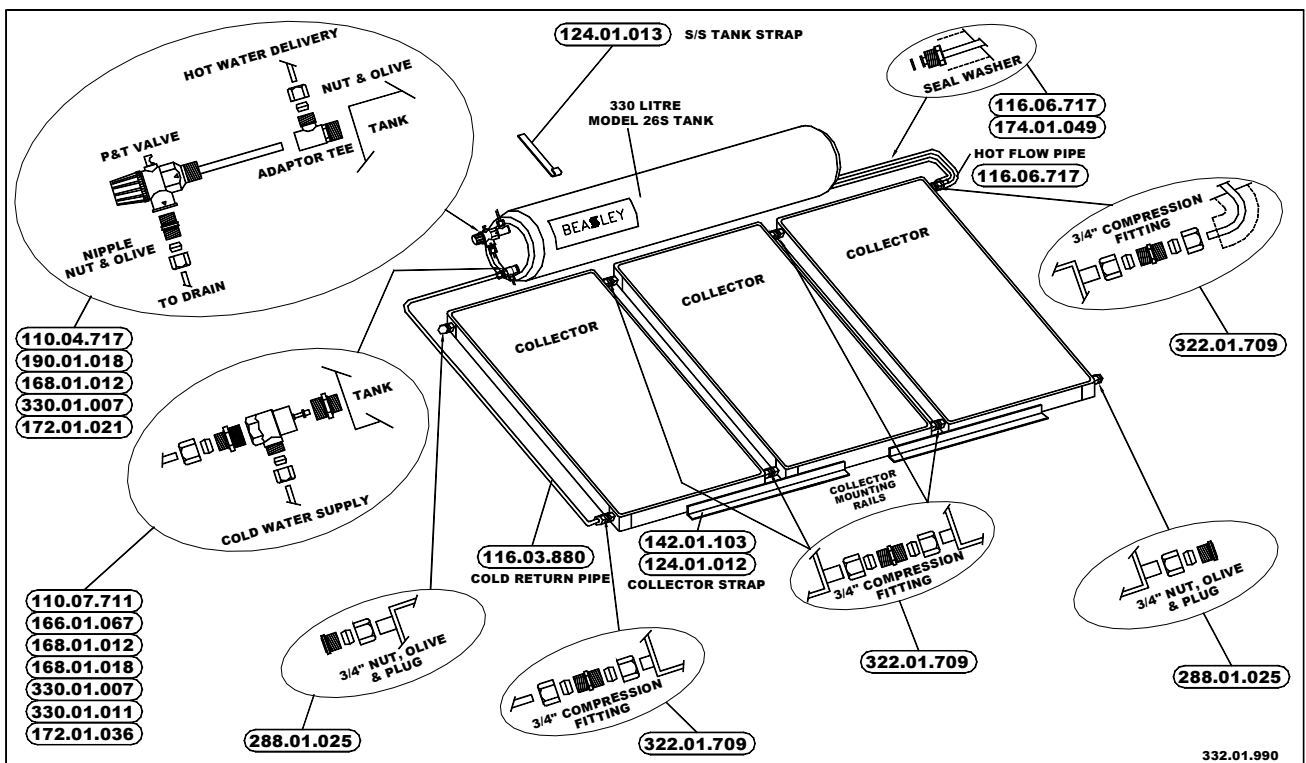
Figure 9. 330 Litre Three Collector System
