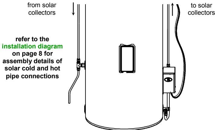
Solar Storage Tank with Solar Control Unit
